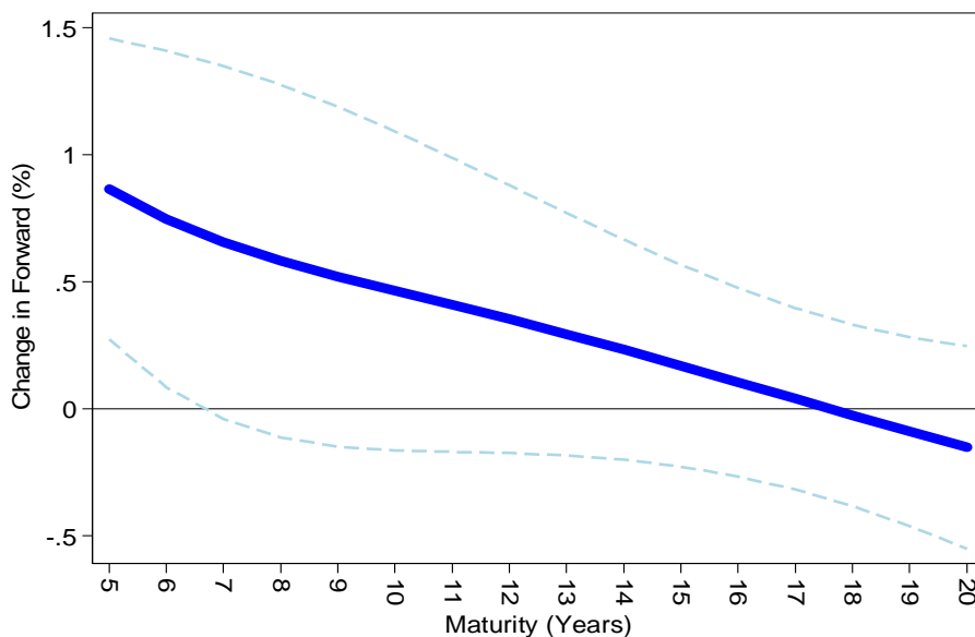
Panel B: Response of real and break-even inflations forwards by maturity
