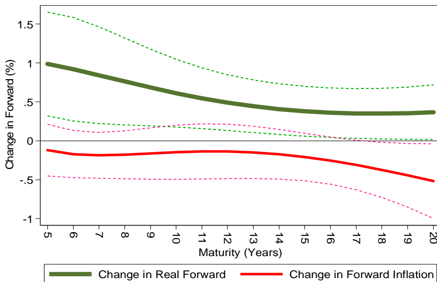
Fig. 3. Instrumental variables estimates of the response of US Treasury forward rates to monetary policy news. Panel A plots the coefficient b_{\S}(n) from instrumental variables (IV) estimation of Eq. (4a) on FOMC announcement dates from 1999 to February 2012:
