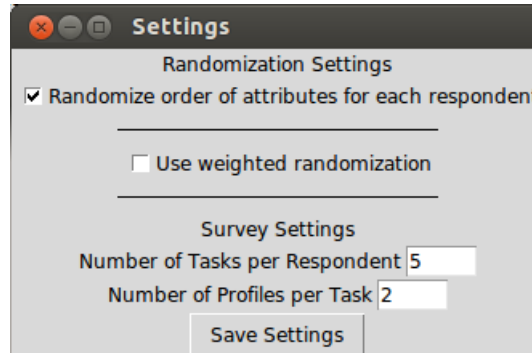
Figure 2: Settings Window
