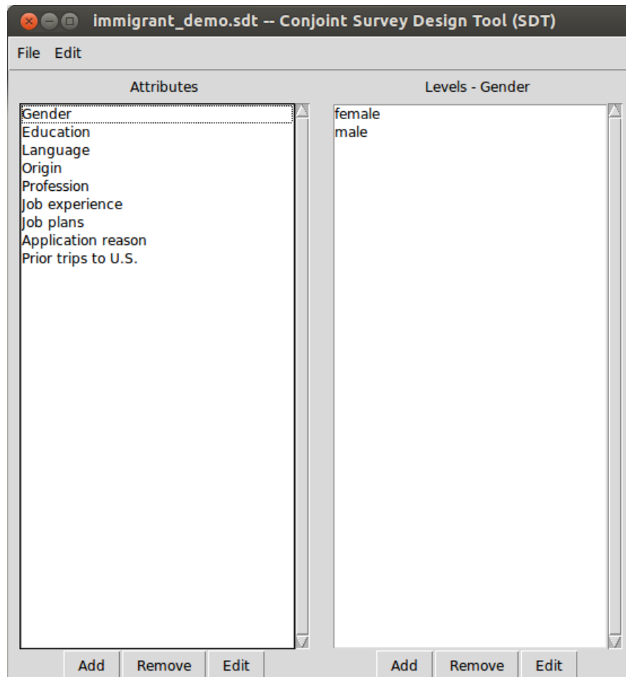
Figure 1: Main Window
