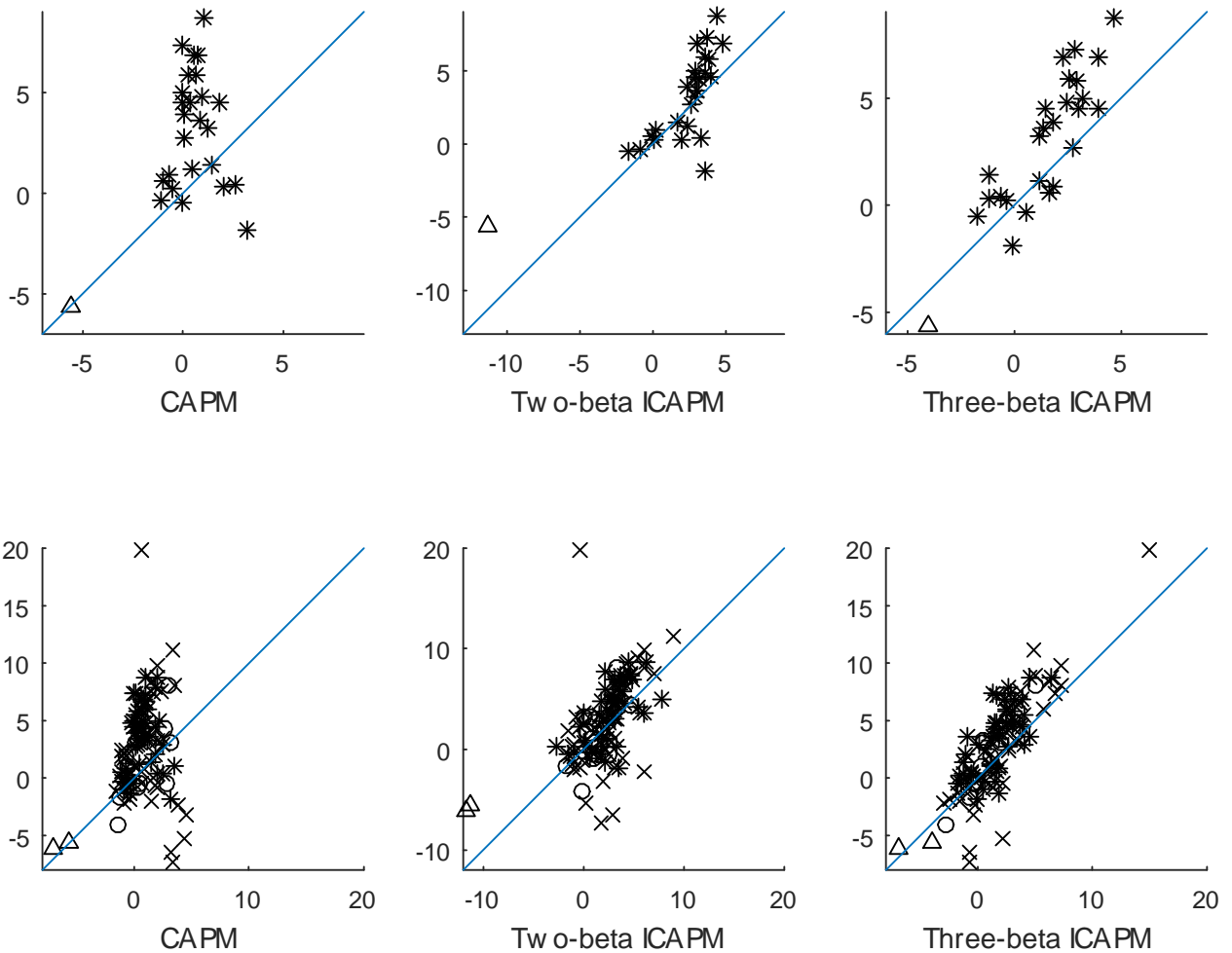
Figure 4: Each diagram plots sample against predicted average excess returns. Test assets in the top row are the 25 ME- and BE/ME-sorted portfolios (asterisks), plus the t-bill return (triangle) and in the bottom row, both unscaled and scaled by EVAR versions of the 25 ME- and BE/ME-sorted portfolios (asterisks), six risk-sorted portfolios (circles), 18 characteristic and risk-sorted portfolios (crosses), and t-bill return (triangles). Predicted values are from Table 4 for 1963:3-2011:4. From left to right, the models tested are the CAPM, the two-beta ICAPM, and the three-beta ICAPM.
