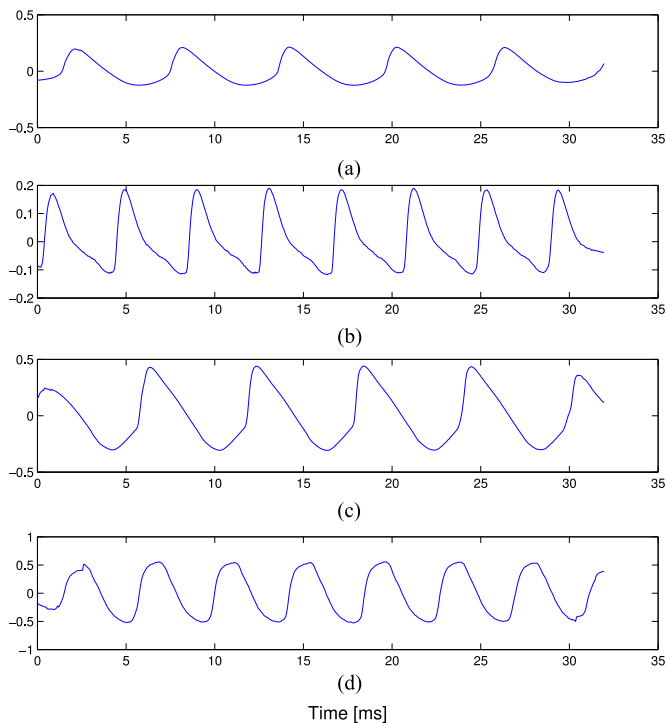
Fig. 6. Prototype electroglottograph speech signal for (a) breathy, (b) modal, (c) strained, and (d) rough quality.
