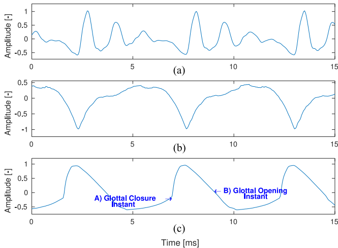
Fig. 1. A 15 ms segment of time-synchronized (a) acoustic, (b) glottal inverse filtered (GIF), and (c) electroglottography (EGG) signals of the vowel /a/ in modal voice quality for a female speaker.
