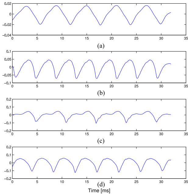
Fig. 5. Prototype glottal inverse filtered signal for (a) breathy, (b) modal, (c) strained, and (d) rough quality.
