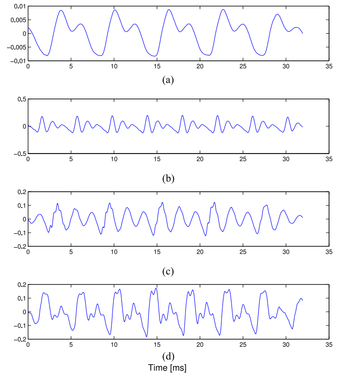
Fig. 4. Prototype acoustic signal for (a) breathy, (b) modal, (c) strained, and (d) rough quality.
