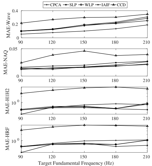
Figure 7. Subset error averages for target fundamental frequencies. Only utterances of vowel /ä/ in the sustained-vowel data set are used.
