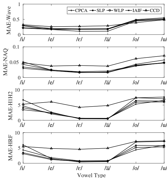
Figure 4. Subset error averages for vowel types.
