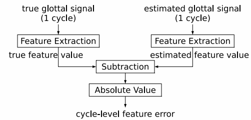
Figure 3. Error evaluation for a particular cycle (identified from the synthesized glottal area signals) and each of the features NAQ, H1-H2, and HRF. For each feature, the median of all cycle-level errors in an utterance is calculated to give a median absolute feature error.
