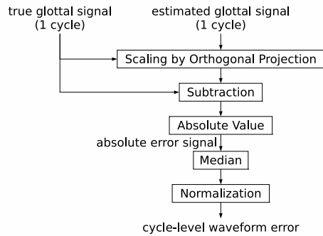
Figure 2. Waveform error evaluation for a particular cycle identified from the synthesized glottal area signals. The median of all cycle-level waveform errors in an utterance is calculated to give an MAE-Wave.
