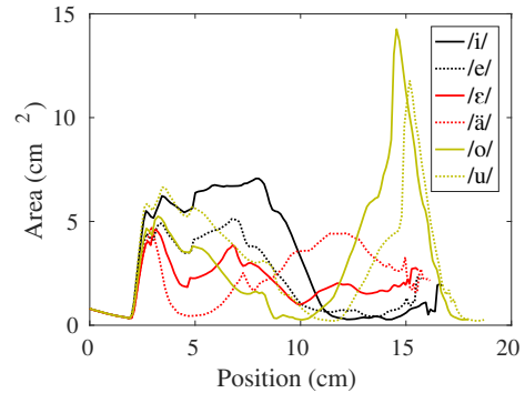
Figure 1. Area functions realizing the 6 sustained vowel types in the experiments. Each function represents the position-varying cross-sectional area of vocal tract, with the glottis being the positional origin.
