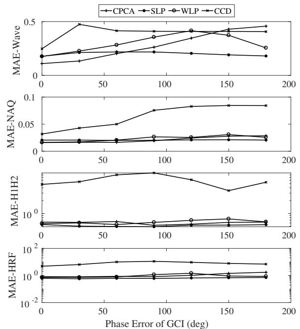
Figure 10. Performance of four algorithms under various amounts of error in each simulated glottal closure instant (GCI) estimate used by the algorithms. Only utterances of vowel /ä/ in the sustained-vowel data set are used in these experiments.
