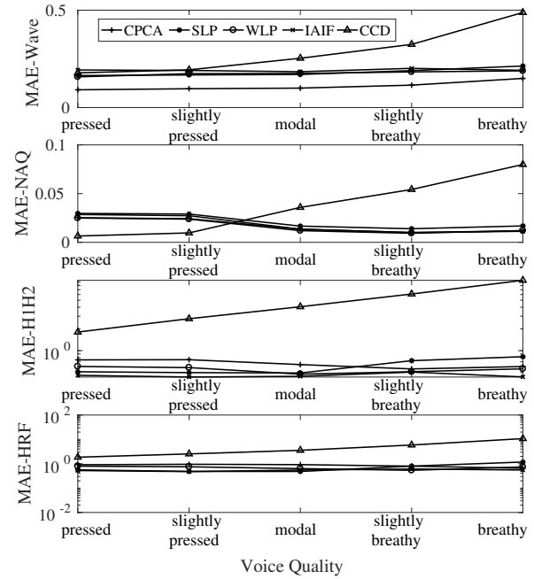
Figure 5. Subset error averages for voice qualities. Only utterances of vowel /ä/ in the sustained-vowel data set are used.
