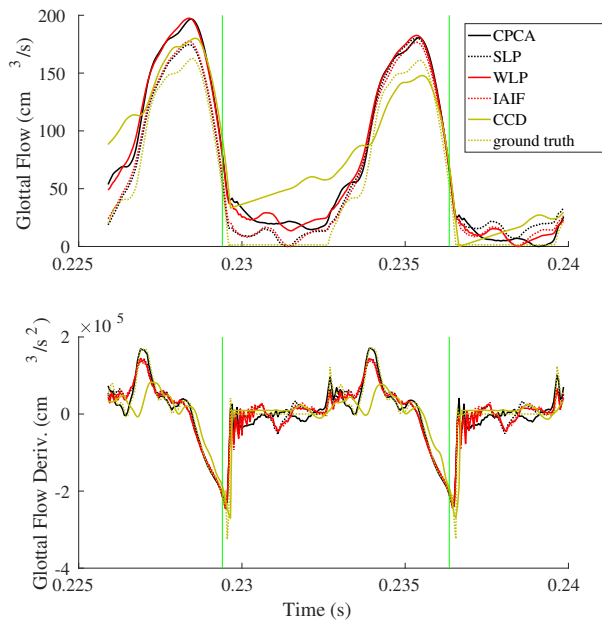
Figure 9. Glottal flow and derivative ( \tilde{\epsilon}_c[n] ) estimates generated by the tested algorithms at the median cycle marked in Fig. 8. The endpoints of the cycle are marked with vertical green lines.
