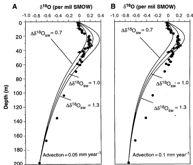
Fig. 3. Comparison of pore fluid data and model calculations for different glacial-interglacial changes in \delta^{18}\text{O}_{\text{sw}} with two different advection velocities: (A) 0.05 \text{ mm year}^{-1} and (B) 0.10 \text{ mm year}^{-1} . For advection greater than 0.05 \text{ mm year}^{-1} , the model curves do not reproduce the \delta^{18}\text{O} -depth gradient that persists to the base of the hole.
