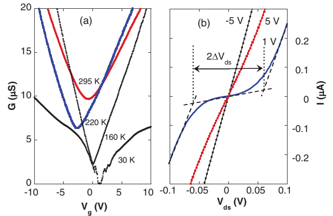
FIG. 4. (Color online) (a) Conductance versus gate voltage measured at various temperatures for sample A. (b) I - V characteristics measured at different gate voltages and at T = 4.3 K for sample A.
