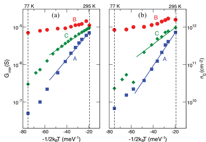
FIG. 3. (Color online) (a) Temperature dependence of the minimum conductance for samples A, B, and C. (b) Temperature dependence of the residual carrier density extracted from the model fitting in Fig. 1 for samples A, B, and C. The solid lines are fits to the simple activated behavior.
