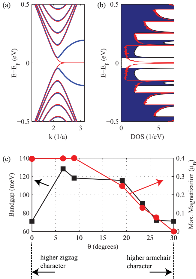
FIG. 6. (Color online) (a) Electronic band structure and (b) density of states of a (3,2)-GNR; results in the absence ( U = 0 eV) and presence ( U = 6.4 eV) of electron-electron correlation are shown in red and blue, respectively. (c) Calculated band gaps (black) and maximum spin magnetization (red) for GNRs of (n,m) -type (6,0), (7,1), (5,1), (4,2), (3,2), and (3,3), corresponding to chiral angles \theta in ascending order.
