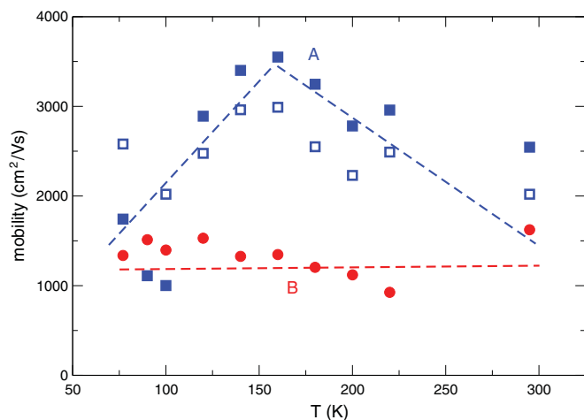
FIG. 2. (Color online) Mobility as a function of temperature for samples A and B. The solid squares and solid circles are the mobility extracted from the model fitting in Fig. 1; the hollow squares are the field-effect mobility. The dashed lines are a guide to the eye.
