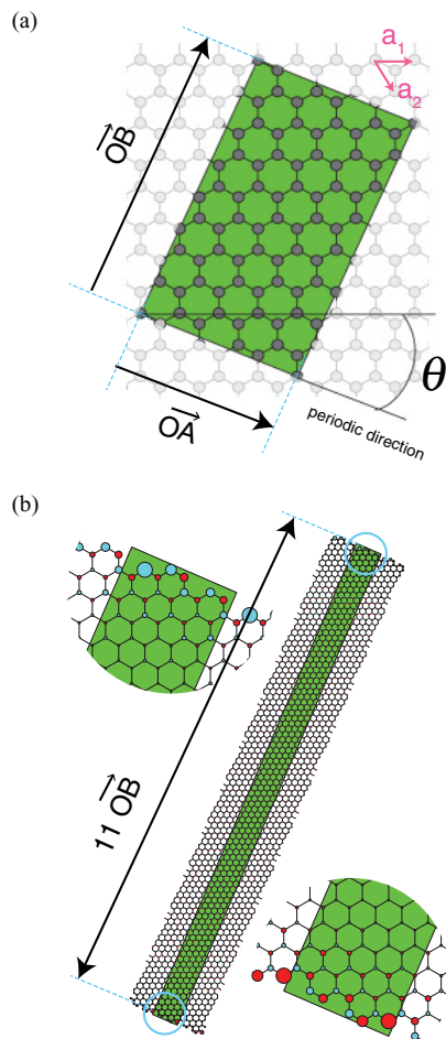
FIG. 5. (Color online) (a) Unrolled projection of a (n,m) -CNT of minimum circumference ( |\vec{OB}| ). The chiral angle \theta is determined by the translational vector \vec{OA} = (n,m) = (3,2) = 3\vec{a}_1 + 2\vec{a}_2 . (b) Cross-section of a (3,2) -GNR with \sim 20 nm width. The periodic unit cell used in the calculation is shown shaded in green. The zoom-in regions show the spatial distribution of spin-up (cyan) and spin-down (red) magnetization. The magnitude of the magnetization is given by the radius size, with the largest radius corresponding to spin magnetization 0.13 \mu_B .
