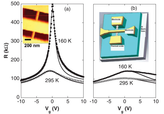
FIG. 1. (Color online) Resistance versus gate voltage for (a) sample A (lower-disorder) and (b) sample B, measured at various temperatures. The solid lines are the model fitting. The two samples belong to a single GNR with uniform width ( W \sim 20 nm) and thickness ( d \sim 1.4 nm), and both have the same length L \sim 600 nm. Insets: schematic illustration of a GNR-FET consisting of a suspended GNR (right) and the contact electrodes and an AFM image of a GNR suspended by Au electrodes (left).
