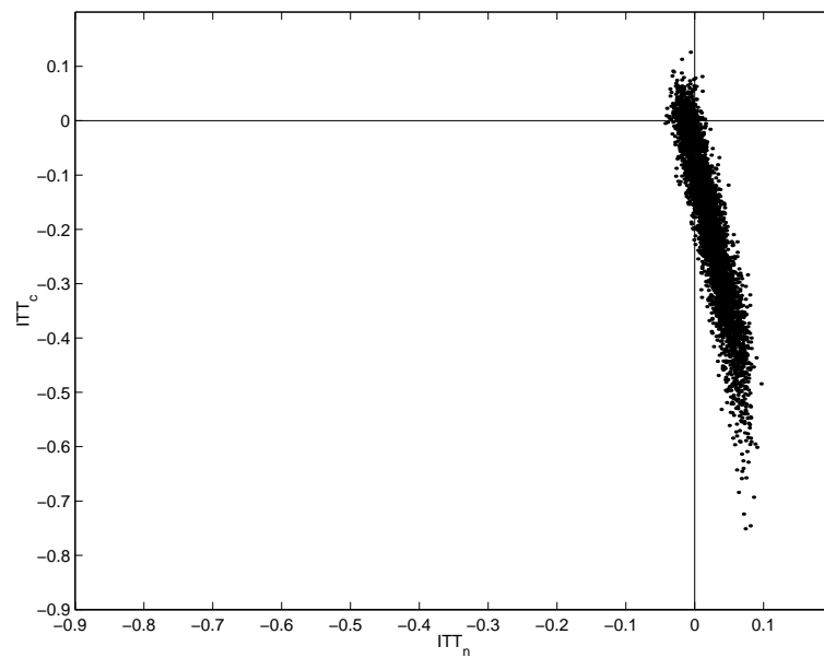
Fig. 2. Simulation scatterplot of the joint posterior distribution of ITT_n and ITT_c , in the model with exclusion restriction only for always-takers.
