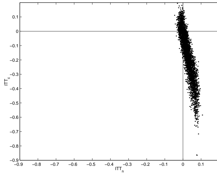
Fig. 4. Simulation scatterplot of the joint posterior distribution of ITT_n and ITT_c , in the model with no exclusion restrictions.
