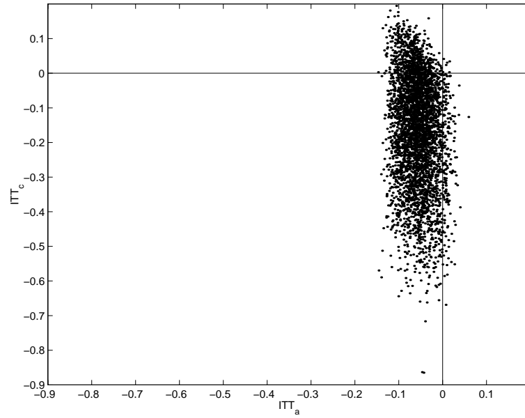
Fig. 3. Simulation scatterplot of the joint posterior distribution of ITT_a and ITT_c , in the model with no exclusion restrictions.
