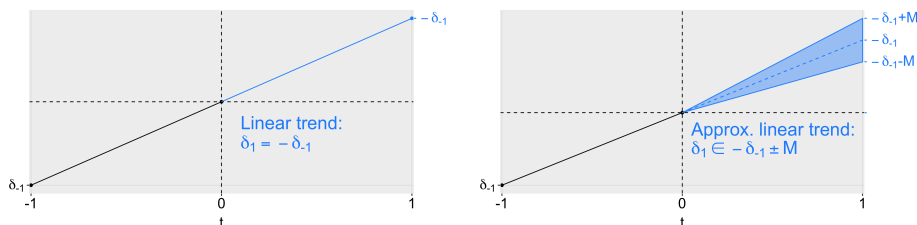
Figure 1: Intuition for \Delta^{SD}(M)
