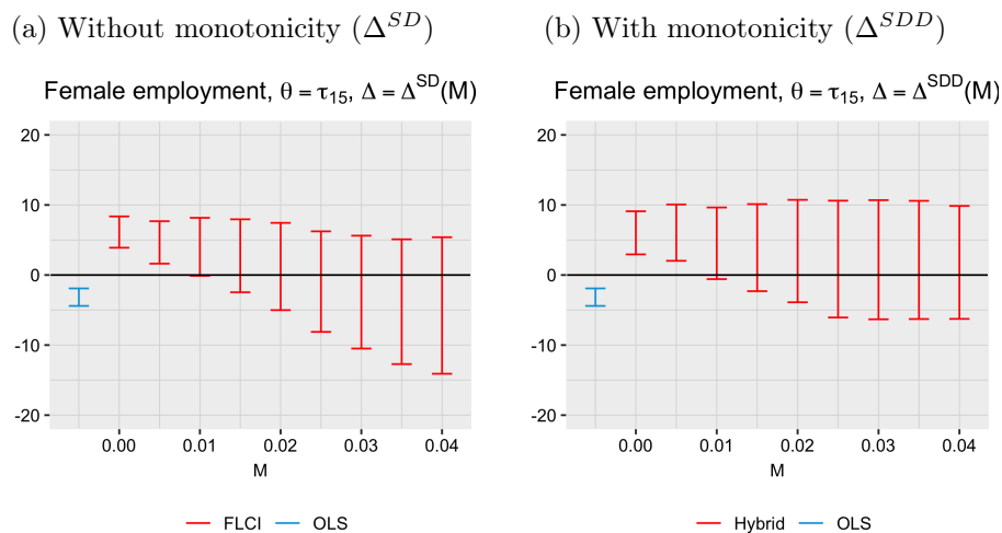
Figure 8: Sensitivity analysis with and without imposing monotonicity
