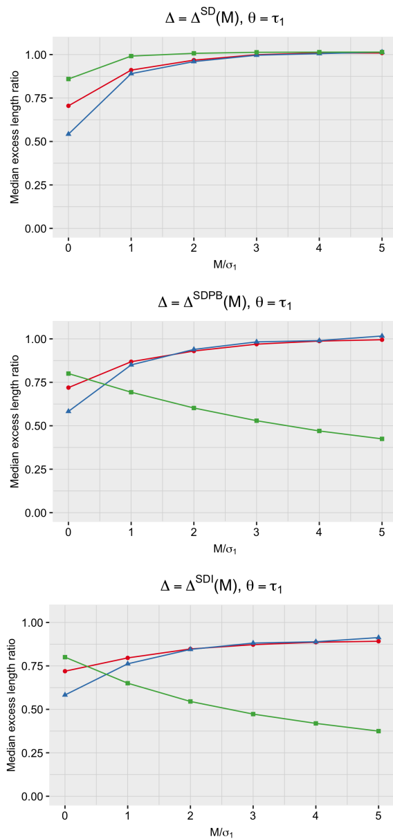
Figure 5: Simulation results: Median efficiency ratios for proposed procedures.
