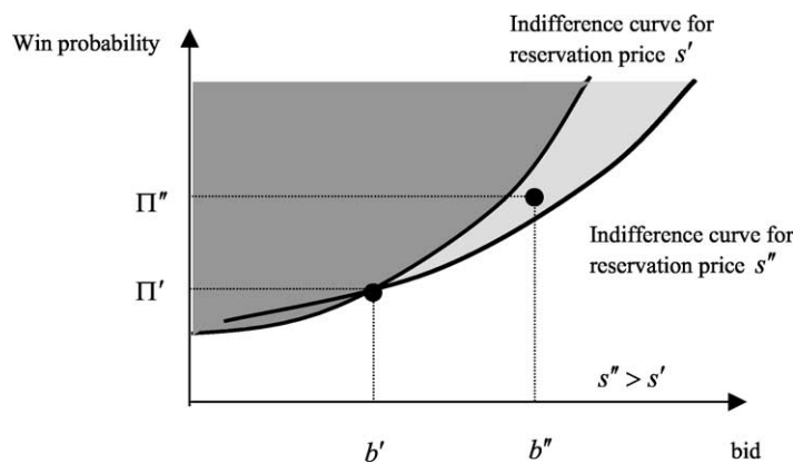
Fig. 1. Single-crossing property.
