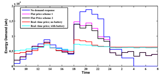
Fig. 6. Electricity demand response under different schemes
