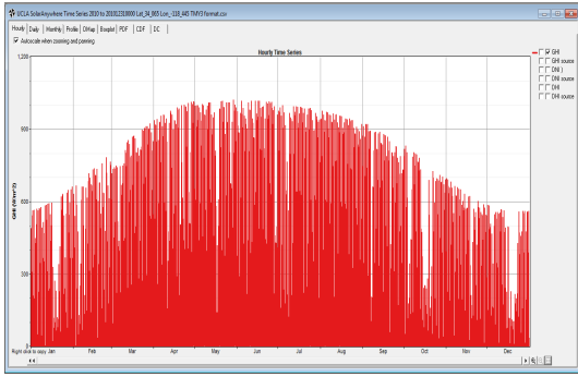
Figure 2. Hourly GHI in 2010 for the UCLA SMERC
