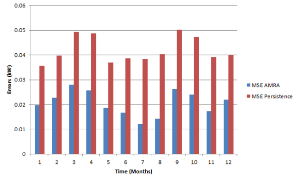
Figure 9. The MSE of the ARMA model and the persistence model for 1 hour-ahead forecasting for each month of 2011 for the UCLA SMERC
