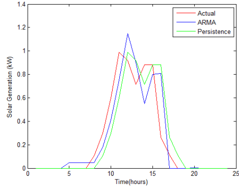
Figure 4. 1 hour-ahead solar generation forecasting and actual data on Jan. 1st, 2011 for the UCLA SMERC
