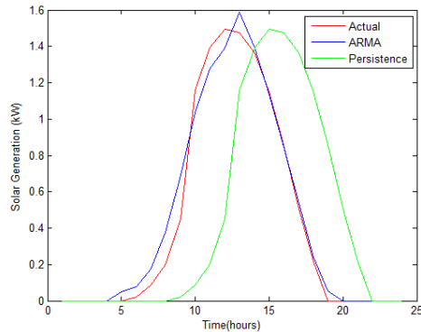
Figure 7. 3 hour-ahead solar generation forecasting and actual data on Jul. 1st, 2011 for the UCLA SMERC
