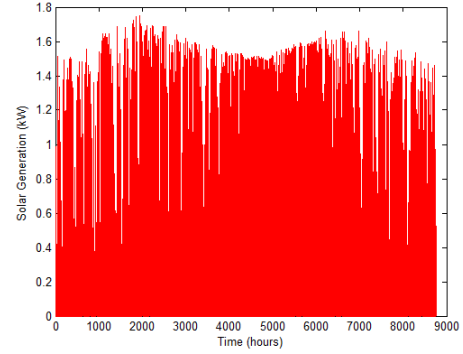
Figure 3. Hourly solar generation simulated by SAM with 1 kW PV in 2010 for the UCLA SMERC
