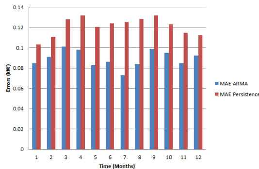
Figure 8. The MAE of the ARMA model and the persistence model for 1 hour-ahead forecasting for each month of 2011 for the UCLA SMERC
