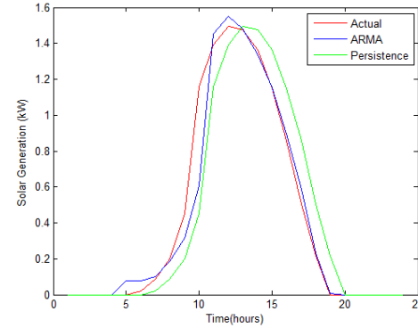
Figure 5. 1 hour-ahead solar generation forecasting and actual data on Jul. 1st, 2011 for the UCLA SMERC
