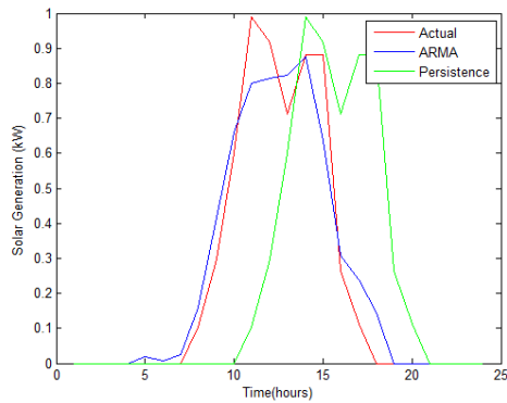
Figure 6. 3 hour-ahead solar generation forecasting and actual data on Jan. 1st, 2011 for the UCLA SMERC
