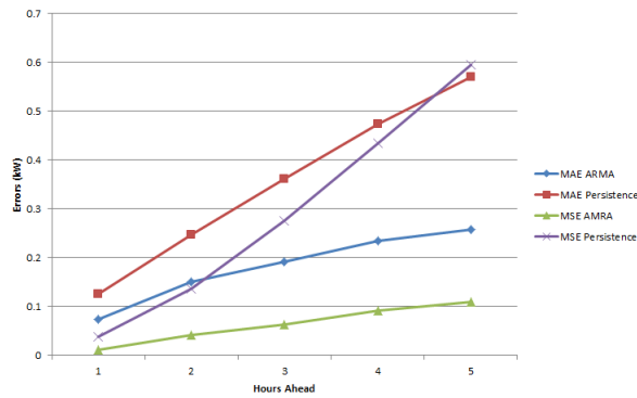
Figure 10. The MAE and MSE of the ARMA model and the persistence model in July, 2011 for different hour-ahead forecasting for the UCLA SMERC
