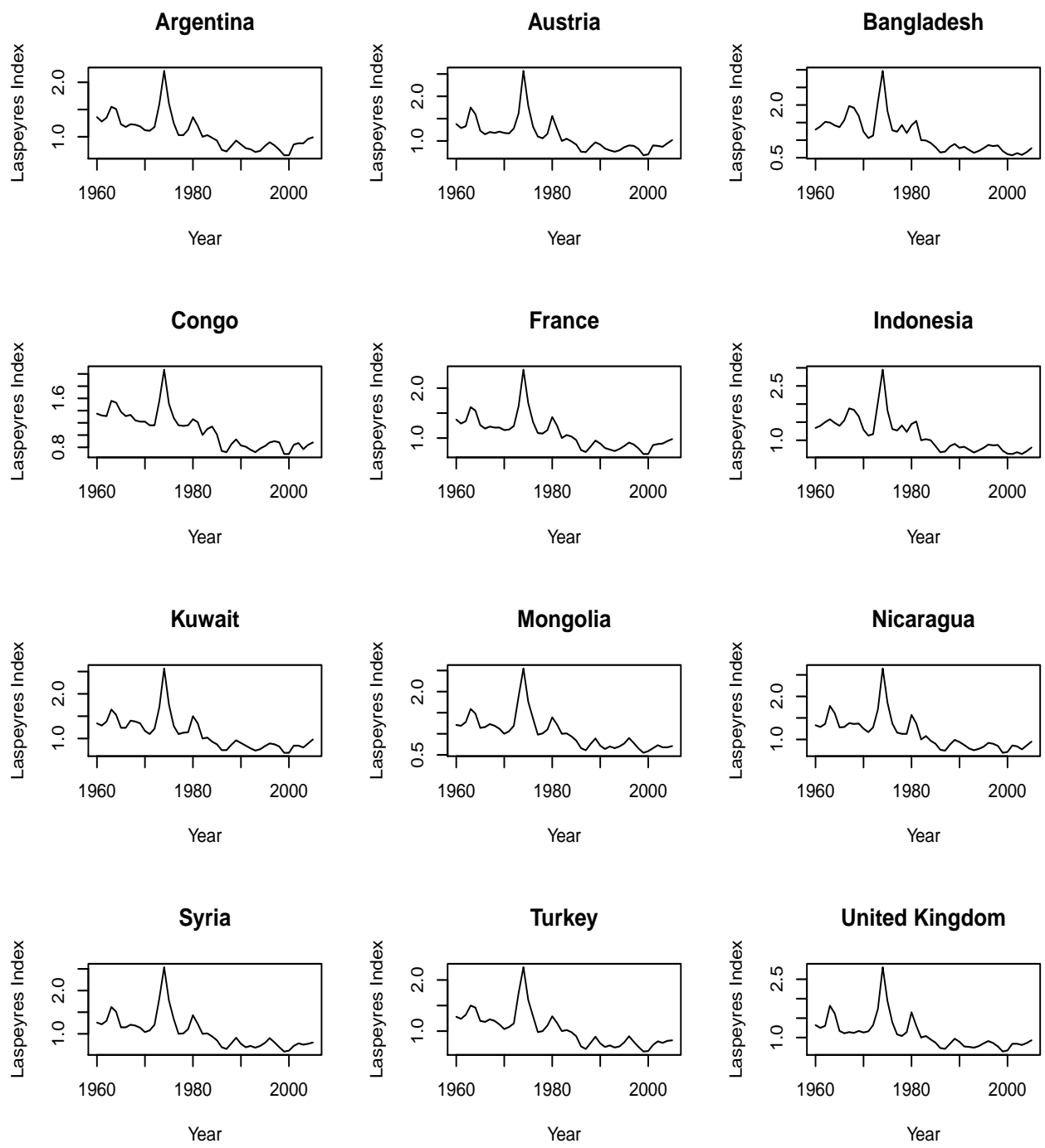
Figure 1: Laspeyres Time Series for a Random Country Sample
