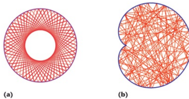
Figure 3. A circular container (left) is non-ergodic while a cardioid container (right) is. If let to continue indefinitely, the left trajectory would never reach the center, while the right trajectory would eventually fill the entire volume.
