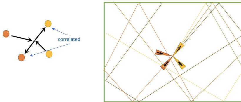
Figure 2. When two molecules collide, the outgoing velocities are correlated. Over time, the correlated velocities spread out to very different regions of phase space.
