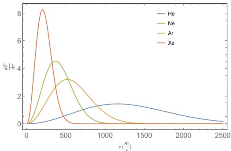
Figure 4. Maxwell-Boltzmann velocity distributions for some gases with the same value of the average energy \bar{\epsilon} = \frac{E}{N} .
