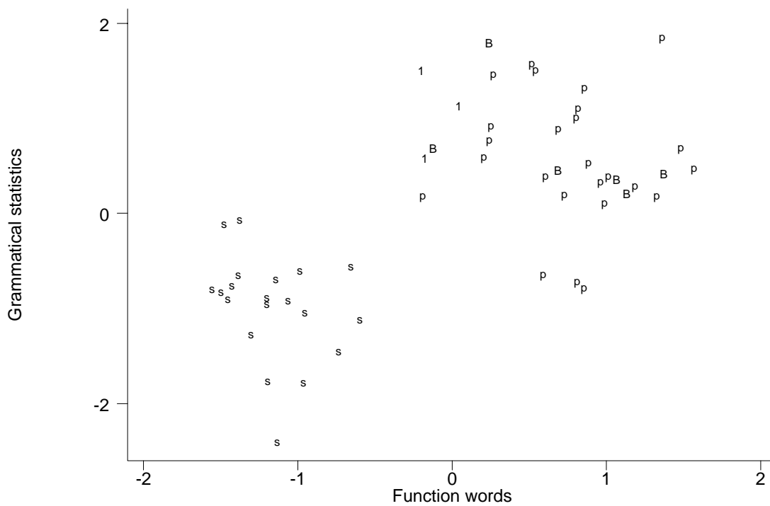
Figure 2 Scatterplot of linear discriminant based on grammatical statistics vs. linear discriminant based on function words.
