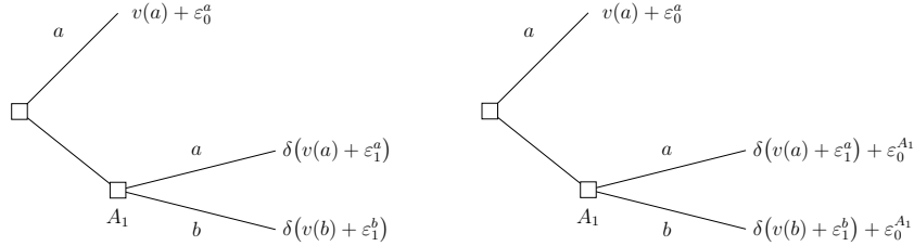
Figure 3: Optimal stopping: Payoffs under BEU (left) vs. DDC (right).
