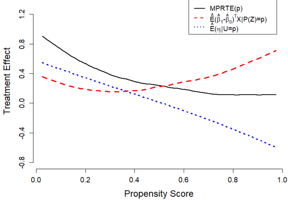
Figure 3: Decomposition of \text{MP RTE}(p) Based on Semiparametric Estimates of \widetilde{\text{MTE}}(p, u) .
