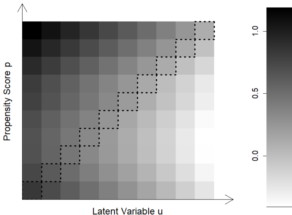
Figure 2: Treatment Effect Heterogeneity based on Semiparametric Estimates of \widetilde{MTE}(p, u) .
