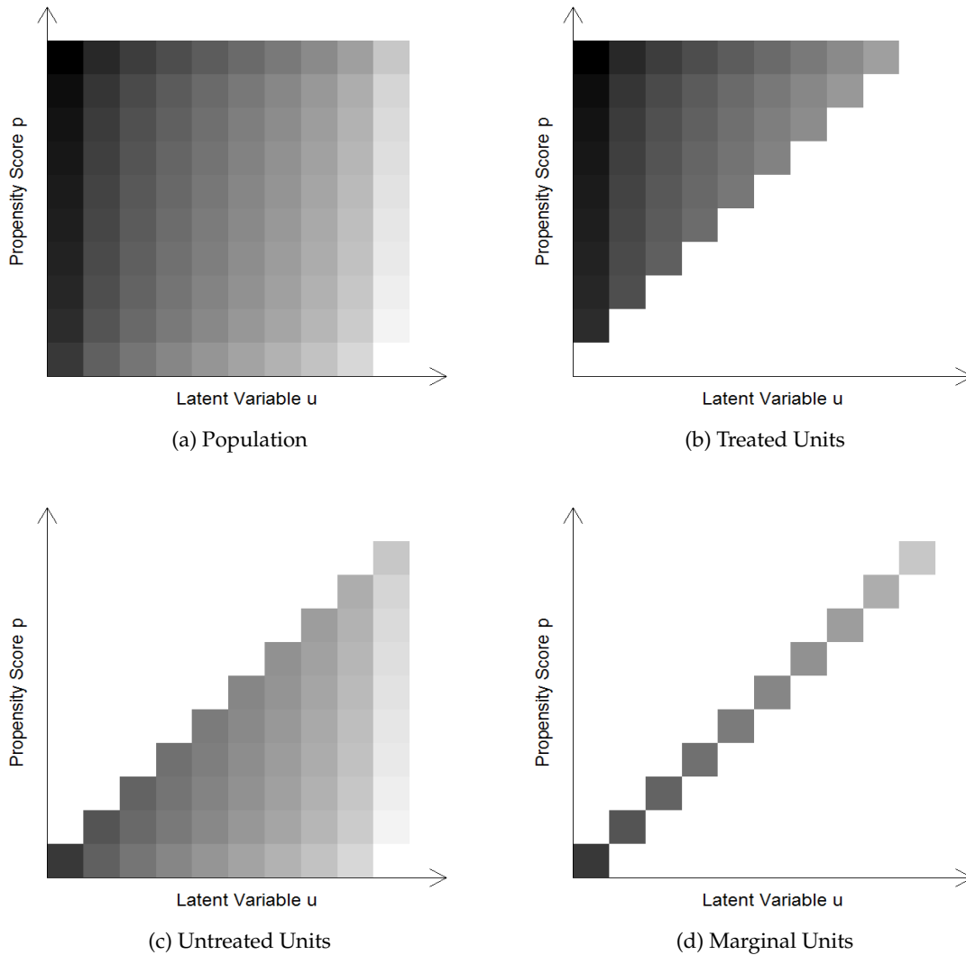
Figure 1: Demonstration of Treatment Effect Heterogeneity by Propensity Score P(Z) and latent variable U . A Darker Color Means a Higher Treatment Effect.
