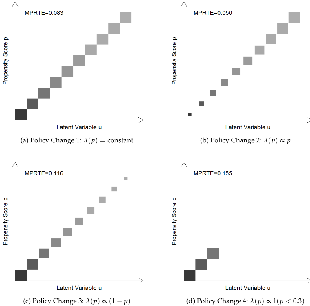
Figure 5: Semiparametric Estimates of MP RTE under Four Policy Changes.
