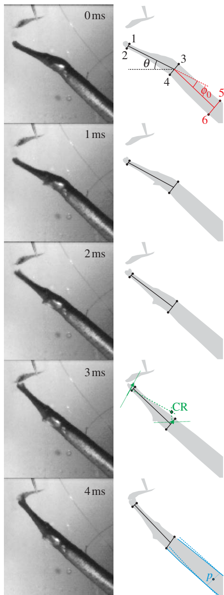
Figure 2. Prey capture sequence of S. leptorhynchus feeding on a mysid shrimp held by forceps. The measured kinematic variables are illustrated on the right: the head angle ( \theta ; black), head to body angle at t=0 ms ( \phi_0 ; red). These angles were calculated based on six landmarks on the pipefish as indicated on the top drawing (1–2, anterior tip of the snout; 3–4, posterior region of the head at the level of the opercular opening; 5–6, approximately one head length further down the body). The determination of the centre of rotation (CR, green) based on the displacement of the upper jaw tip and the dorsal edge of the operculum between t=0 and 3 ms is illustrated in the drawing of t=3 ms. Point p (blue) is the mid-sagittal landmark on the pipefish's body where the ventral movement by the body during dorsal head rotation is approximately negligible. This point was determined from dorsal and ventral body contour tracings of the first frame ( t=0 ms) and the frame at t=4 ms of the high-speed video by taking the xy -average of the points on the body where the corresponding contour lines have converged.
