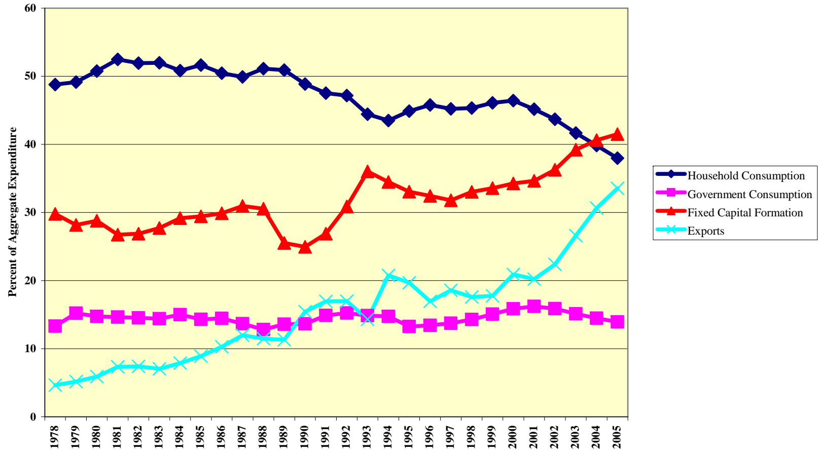
Figure 20.5 Principal Components of GDP Expenditure, 1978-2005
