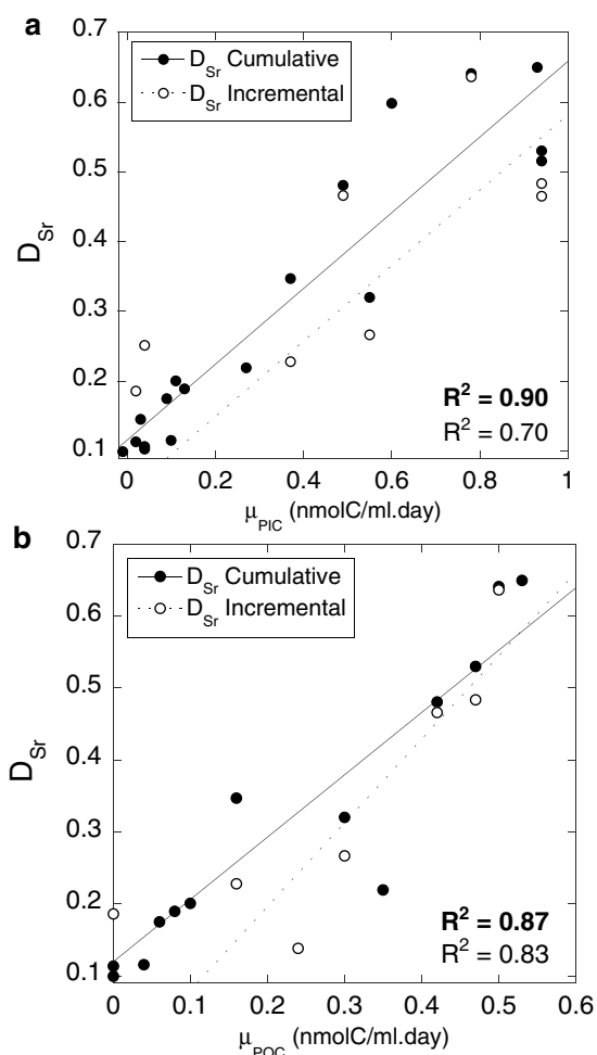
Figure 2. The cumulative (solid circles and solid line) and incremental (open circles and dashed line) strontium partition coefficient ( D_{\text{Sr}} ) plotted against (a) \mu_{\text{PIC}} (cell-specific growth rate of particulate inorganic carbon) and (b) \mu_{\text{POC}} (cell-specific growth rate of particulate organic carbon). A linear best fit yields, for \mu_{\text{PIC}} , an r^2 = 0.90 and 0.70 for cumulative and incremental and, for \mu_{\text{POC}} , r^2 = 0.87 and 0.83 for cumulative and incremental, respectively.
