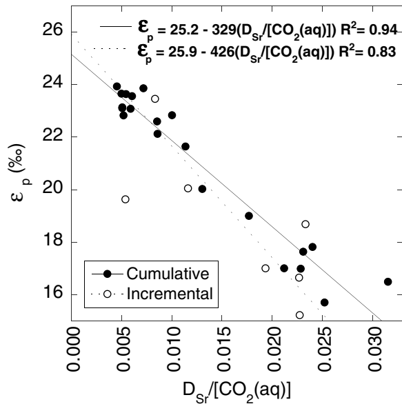
Figure 3. D_{Sr} (partition coefficient of Sr) normalized to [CO_2(aq)] and plotted against \epsilon_p to investigate how well D_{Sr} acts as a proxy for \mu_C , the carbon-specific growth rate. Cumulative values of D_{Sr} and \epsilon_p are plotted in solid circles and with a solid line, and incremental values of D_{Sr} and \epsilon_p are plotted with open circles and a dashed line.
