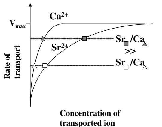
Figure 4. A hypothetical plot of rate of transport of an ion by a carrier protein versus the concentration of the transported ion for Ca^{2+} (triangles) and Sr^{2+} (squares). The slightly higher charge density of the calcium ion relative to the strontium ion leads to stronger bonding of the calcium ion by the protein and more efficient transport at lower concentrations. As the rate of transport of ions increases from the open symbols to the shaded symbols, the Sr/Ca of the transported ions will also increase as marked by the dotted lines.
