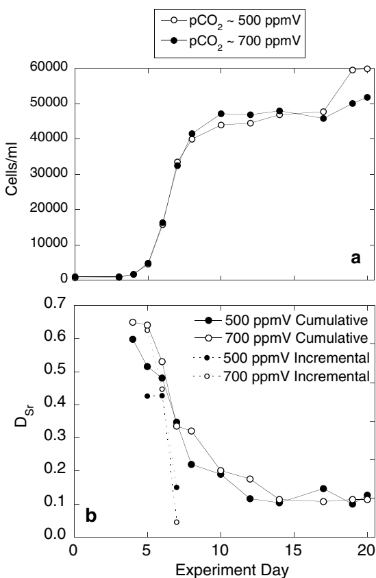
Figure 1. (a) Cell density and (b) the cumulative (solid lines) and incremental (dashed lines) partition coefficient of Sr into the coccoliths ( D_{\text{Sr}} ), plotted versus time (in days) in the two mesocosms with initial p\text{CO}_2 \sim 500 ppmv (open circles) and p\text{CO}_2 \sim 700 ppmv (solid circles). The incremental D_{\text{Sr}} is not plotted during the stationary phase because growth rates are essentially zero and so therefore is the incremental D_{\text{Sr}} . The cumulative data do not incur this problem as the asymptote represents an integral of all coccoliths grown throughout the experiment.
