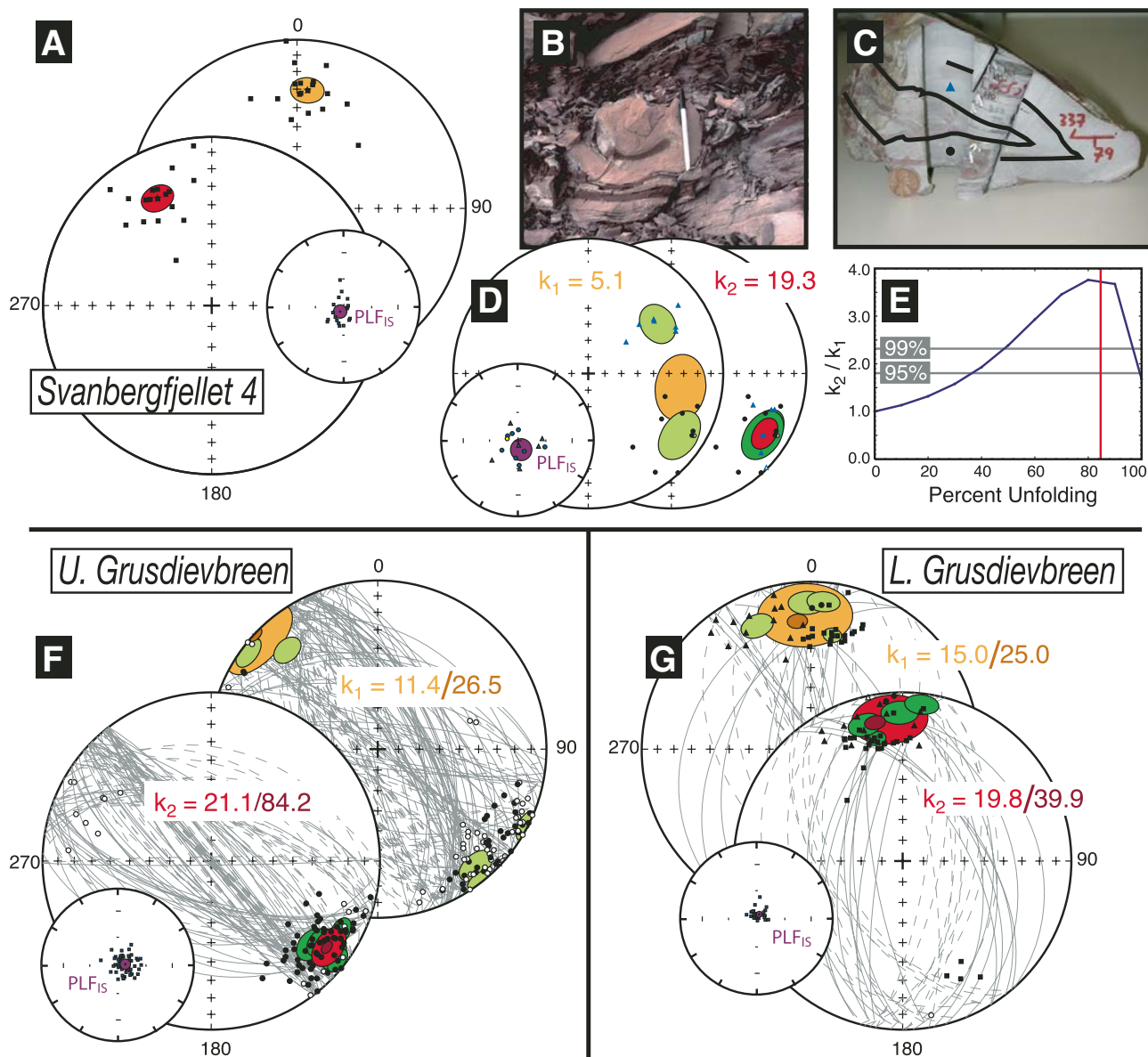
Figure 6. Tests for the presence of pre-folding or synfolding magnetization. Equal-area nets show in situ (orange) and tilt-corrected (red) Fisher distributions of the characteristic remanent magnetization (ChRM) direction and in situ distribution of the present-local field (PLF) overprint (purple) for the Lower Grusdievbreen (IGfm) (G), Upper Grusdievbreen (uGfm) (F), and Svanbergfjellet (S4mb) (A). Filled/open circles are lower/upper-hemisphere least-squares line fits to demagnetization curves. Gray arcs are great circle fits to demagnetization curves with overlapping magnetic components. Where multiple stratigraphic sections are present, as in (F) and (G), individual section-mean Fisher statistics are plotted as light green (in situ) and dark green (tilt-corrected) ellipses, while the averages of section-mean directions are plotted as dark orange (in situ) and dark red (tilt-corrected) ellipses. Values k_1 and k_2 are in situ and tilt-corrected Fisher (Fisher, 1953) concentration parameters measuring the dispersion in individual paleomagnetic data (light orange and light red) and site-mean paleomagnetic data (dark orange and dark red). S4mb contains numerous disturbed beds of pink limestone and red marl with detached syndepositional folds (B) and erosional truncations (left of the pen cap in B). Paleomagnetic directions from the upper limb (blue triangles) and lower limb (black circles) of the fold pictured in C are plotted on the equal-area net in D. The PLF overprint direction fails the fold test, while the primary magnetic component passes the syndepositional fold test at the 99% confidence level (E). (E) Shows that k_2/k_1 is maximized at 86% unfolding and that the S4mb ChRM was likely acquired prior to, or at the onset of slump folding, and thus dates from the time of sedimentation. (Note: the demagnetization behavior of the ChRM from A and D is identical, and the two directions are considered to reflect the same paleomagnetic component. The difference in absolute direction of the ChRM in D with respect to the ChRM in A is just another reflection of the observation that the ChRM was acquired prior to disruption and folding.) Both the uGfm (F) and IGfm (G) directions were derived from multiple stratigraphic sections separated by >100 km. Although paleomagnetic directions are subparallel to the NNW-trending Caledonian fold axes, k_2/k_1 is maximized at 100% unfolding, and both uGfm and IGfm pass the McElhinny (1964) fold test at greater than the 92% confidence level.
