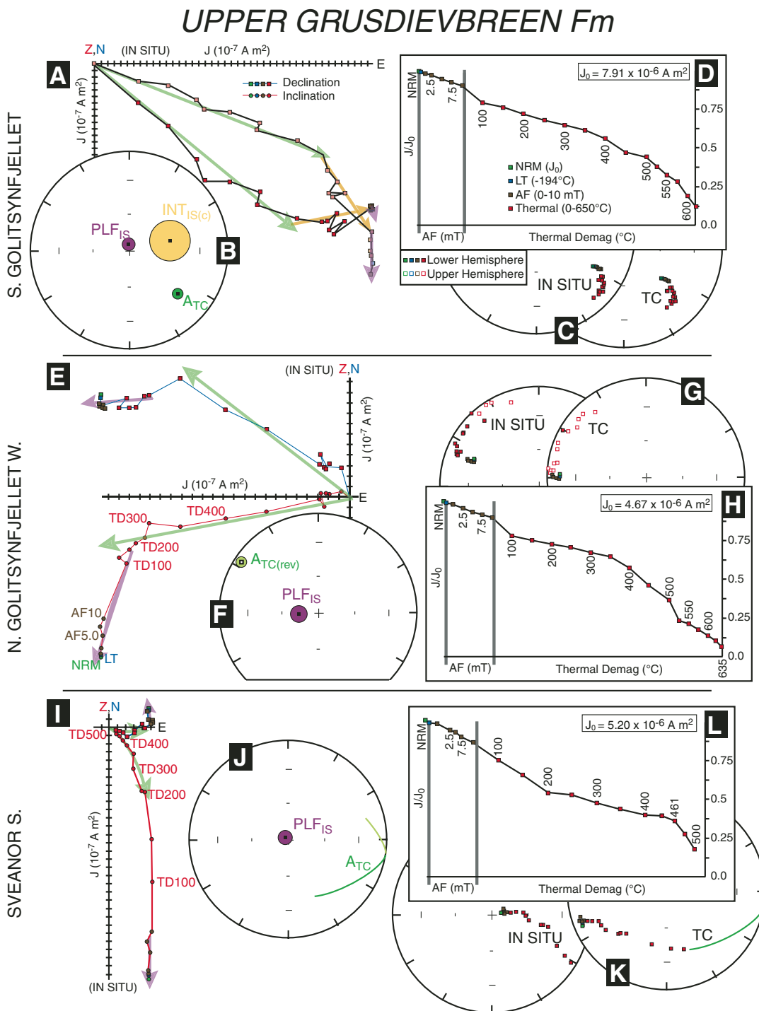
Figure 4. Representative vector component diagrams (Zijderveld, 1967) (A, E, and I), least-squares fits (B, F, and J), equal-area projections (C, G, and K) and magnetic intensity ( J/J_0 ) plots (D, H, and L) showing demagnetization behavior for the Upper Grusdievbreen Formation (uGfm). In the Zijderveld plots (always in situ coordinates), the primary, high-temperature component that decays to the origin is traced with a green arrow, intermediate directions, when present, are traced with a yellow arrow, and the present local field (PLF) overprint is traced with a purple arrow. When thermal unblocking spectra are arcuate, rather than linear, a great circle is fit to the data instead of a line (I–K). Least-squares fits of these components, with error ovals representing circular maximum angular deviation (MAD) angles from the principal component analysis (plotted using the routines of Cogné [2003] and Jones and Tetreault [2004]), are summarized in an adjacent equal-area projection (B, F, and J), and are labeled A TC , INT IS(c) , and PLF IS , respectively, where TC refers to tilt-corrected and IS refers to in situ coordinates. In all plots, green-filled shapes are natural remanent magnetization (NRM) directions, blue-filled shapes are the low-temperature step, brown-filled shapes reflect alternating field (AF) demagnetization steps, and red-filled shapes reflect thermal demagnetization. In the Zijderveld plots (A, E, and I), squares/circles represent declination/inclination, while in the equal-area nets (C, G, and K), color-filled/color-rimmed squares represent lower/upper-hemisphere directions.
