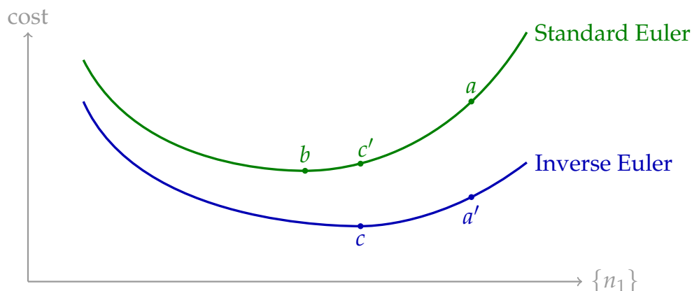
Figure 1: Efficiency gains as a function of n_1 for given v . The upper (green) curve imposes free savings. The lower (blue) curve implements the Inverse Euler equation with optimal savings distortions.
