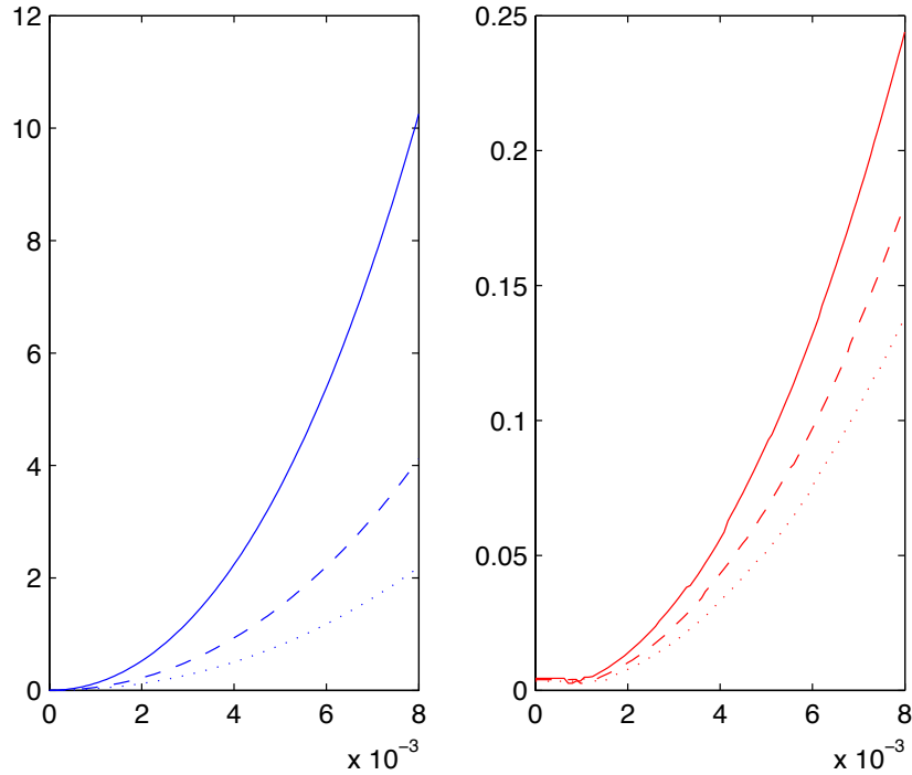
Figure 2: Efficiency gains in % when baseline consumption is a geometric random walk for consumption and the Euler equation holds as function of \sigma_\varepsilon^2 . The left panel shows the gains in partial equilibrium and the right panel shows the gains in general equilibrium. The bottom dotted line corresponds to \beta = .96 , the middle dashed line to \beta = .97 and top plain line to \beta = .98 .
