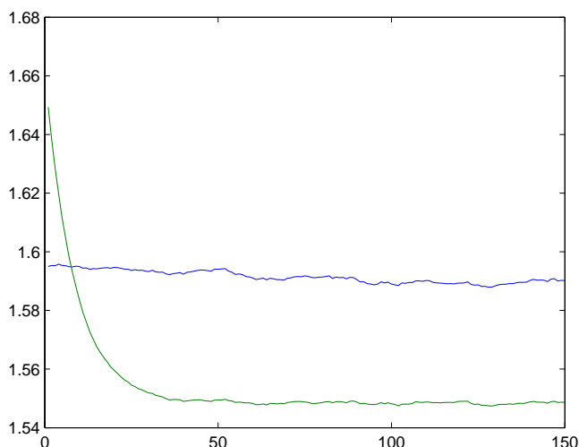
Figure 3: Simulated path of aggregate consumption for the baseline and the optimized allocations for \sigma = 1 , \text{Std}(\log(n_t) - \log(n_{t-1})) = .4 and \rho = 0.9 .
