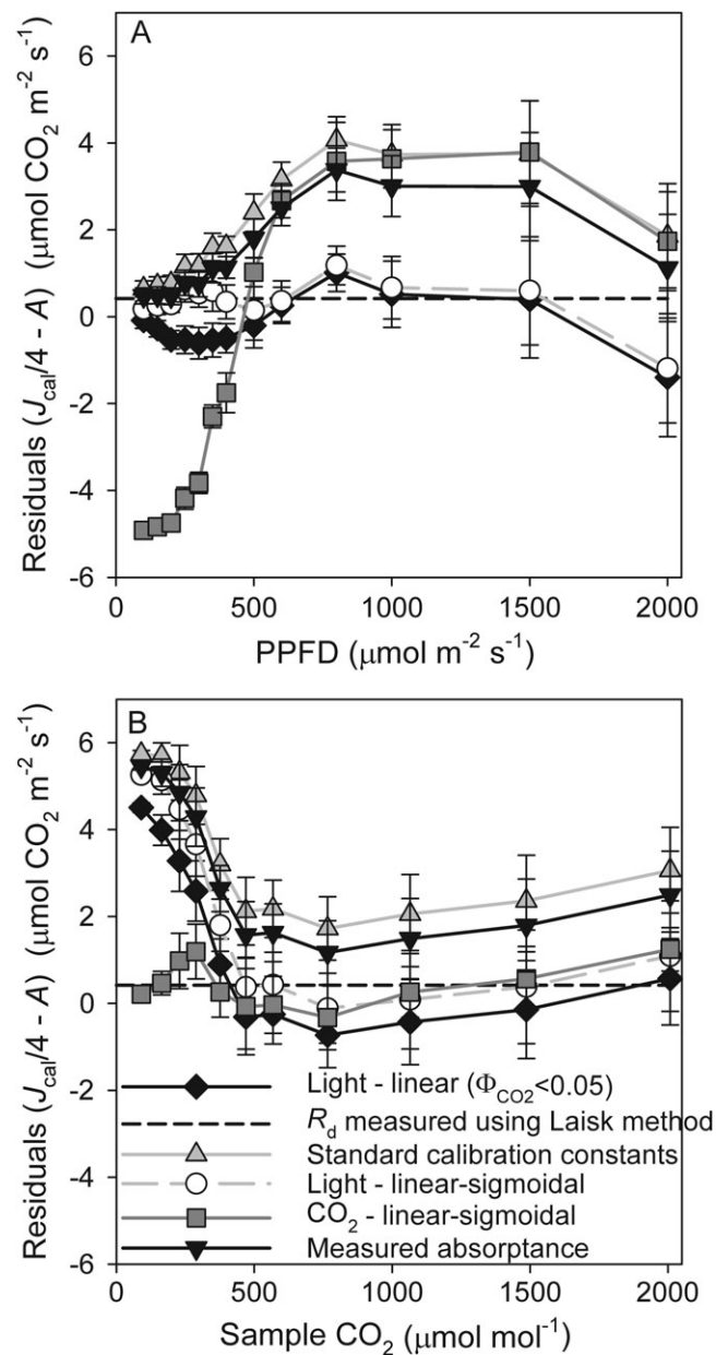
Fig. 2. The average residuals of the calibrated rate of electron transport ( J_{\text{cal}} ), rescaled to units of CO 2 uptake, relative to the observed photosynthetic rate for light (A) or CO 2 response curves (B) measured under non-photorespiratory conditions. To allow for possible trends in R_d , residuals were calculated as J_{\text{cal}}/4 - A . Points represent the mean and standard errors for five or more replicate light curves (the same data as in Fig. 1A and C) or five CO 2 response curves (the same data as in Fig. 1B and D).
