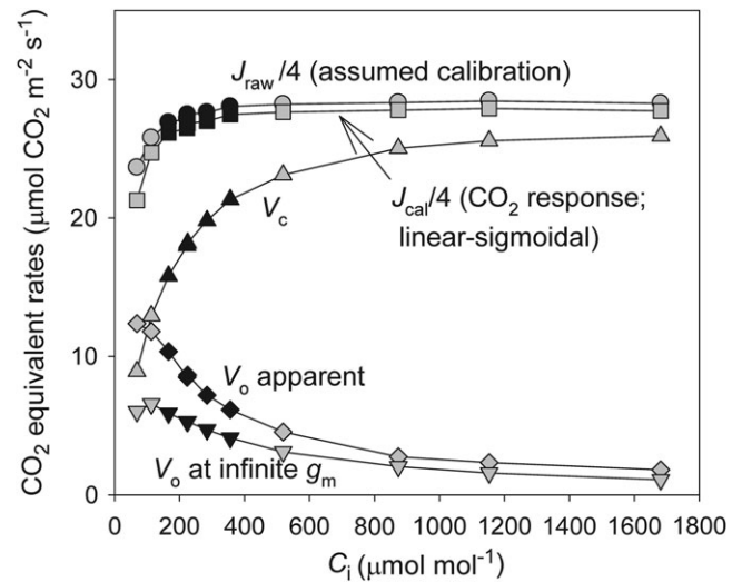
Fig. 6. Rates of the standard fluorescence estimate of electron transport ( J_{\text{raw}} ), the calibrated rate of electron transport expressed in CO 2 equivalents, carboxylation ( V_c ), apparent photorespiration rate ( V_o apparent = J_{\text{cal}}/4 - V_c ), and photorespiration calculated assuming C_c = C_i ( V_o at infinite g_m ), for a measured response to CO 2 . Note the small shift in V_o necessary to result in an infinite g_m at high CO 2 . Points that satisfy the Harley criterion (filled symbols) and those that did not (open symbols) are distinguished. Experimental conditions were the same as in Fig. 3.
