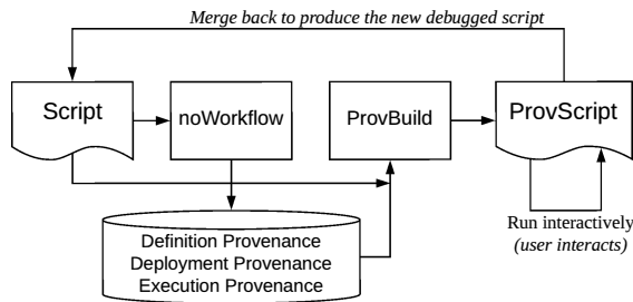
Figure 1: ProvBuild Architecture.
