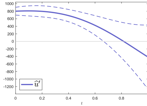
Notes: This graph shows point-wise 95% credible sets for u' .
