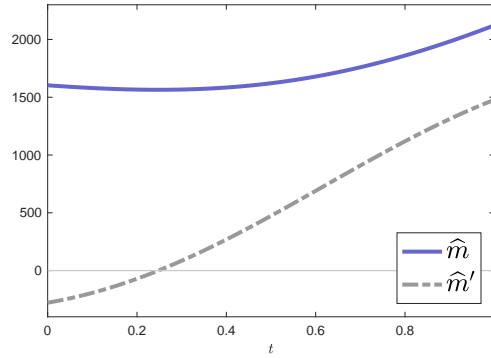
Notes: This graph shows our estimate of m , which describes average health care expenditures as a function of the subsidy rate t , and our estimate of m' .
