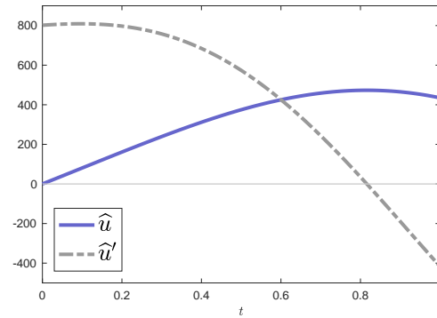
Notes: This graph shows our estimate of u , which describes social welfare as a function of t , and our estimate of u' .
