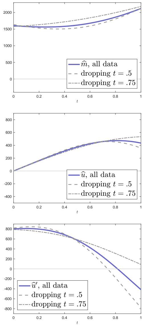
Figure 3: Robustness of interpolation
