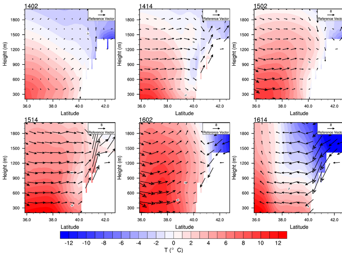
Fig. 5. Simulated N-S vertical cross sections of 12-hourly v-w wind components (vectors, m/s) and temperature (contours, °C) in the NCP along 116.4°E during February 14–16, 2017. The v wind component is multiplied by 100.
