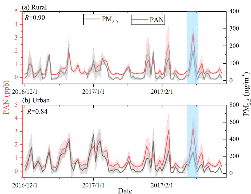
Fig. 1. Observed daily concentrations of PAN (ppb) and PM 2.5 (µg/m 3 ) at the rural (a) and urban sites (b) during winter of 2016–2017. The standard deviation is calculated by the hourly data and displayed by shades. Blue rectangular shades denotes the simulation periods in this study. (For interpretation of the references to color in this figure legend, the reader is referred to the web version of this article.)
