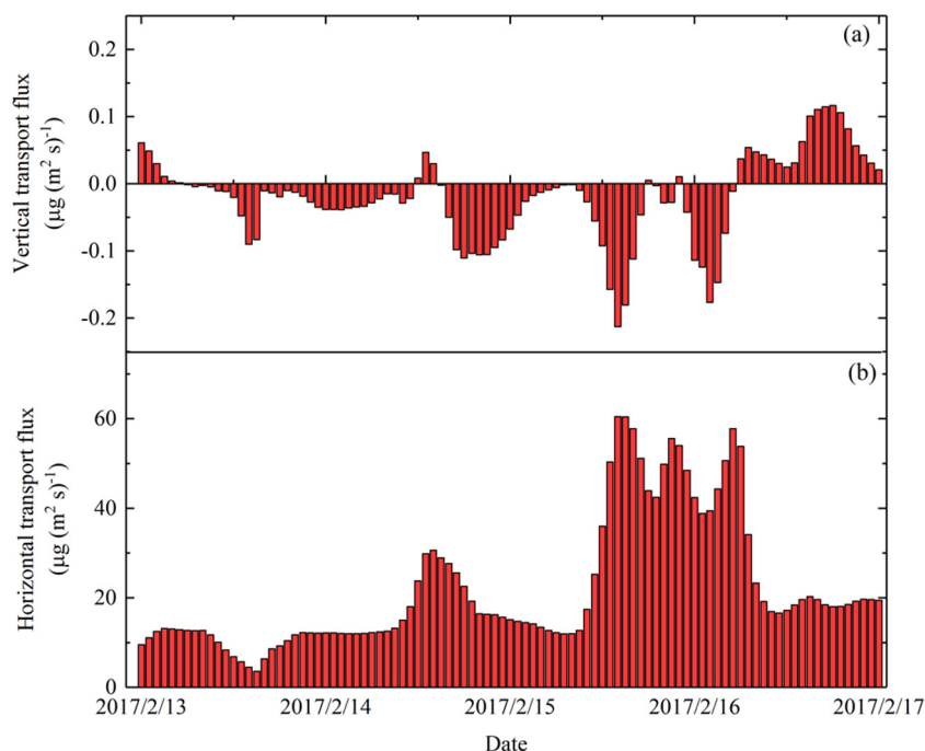
Fig. 7. Simulated time series of the vertical and horizontal transport flux ( \mu\text{g m}^{-2} \text{s}^{-1} ) averaged within the 1.2 km layer above the ground in urban Beijing during February 13–16, 2017.
