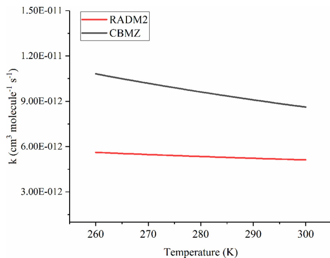
Fig. 4. Simulated reaction rate coefficients for the PAN formation through \text{CH}_3\text{C}(\text{O})\text{O}_2 radicals and \text{NO}_2 in the function of temperature using the RADM2 and CBM-Z schemes.
