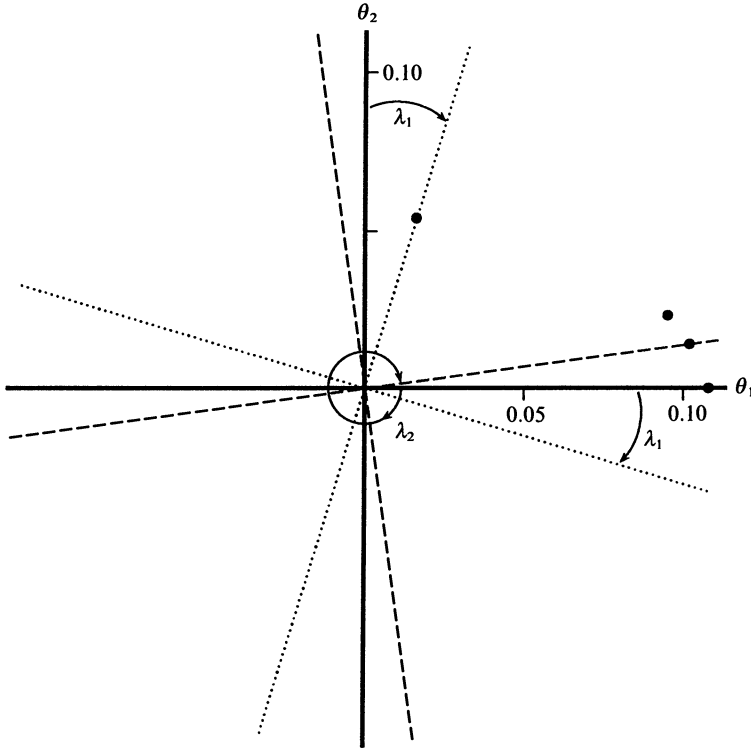
FIGURE 2 Factor rotation
