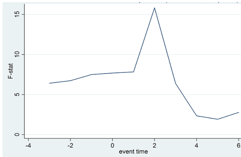
Panel B: SO 2
