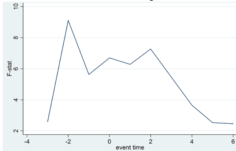
Panel C: NO 2
