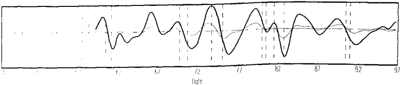
Fig. 3.15. Investment (equipment).
