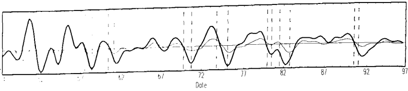
Fig. 3.13. Consumption (durables).
