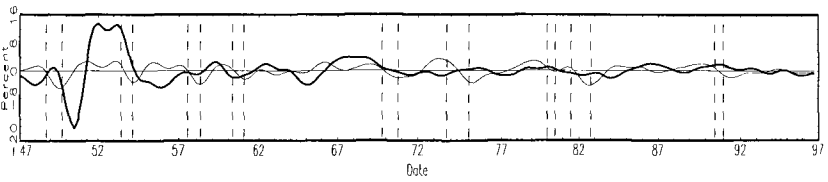
Fig. 3.22. Government purchases.
