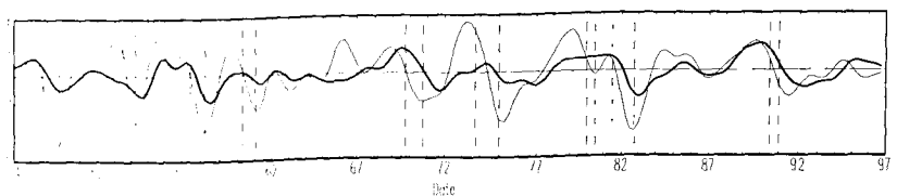
Fig. 3.6. Service employment.
