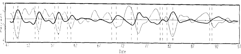
Fig. 3.28. Unemployment rate.
