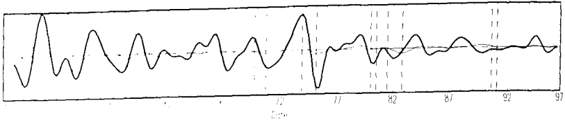
Fig. 3.63. Vendor performance.
