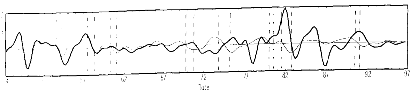
Fig. 3.4. Mining employment.
