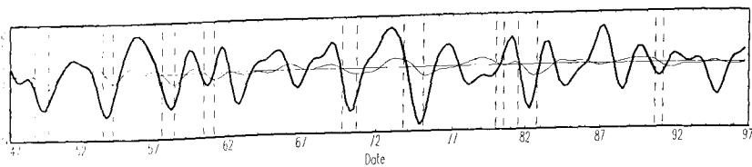
Fig. 3.53. Stock prices.
