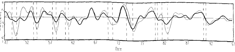
Fig. 3.10. Consumption (nondurables).
