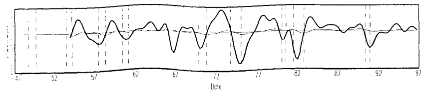
Fig. 3.62. Building permits.
