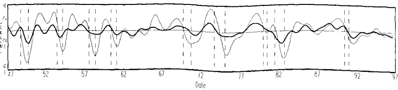
Fig. 3.11. Consumption (services).
