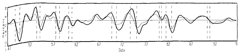
Fig. 3.2. Manufacturing employment.
