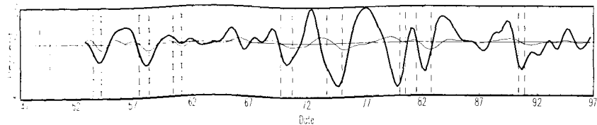
Fig. 3.61. Consumer expectations.
