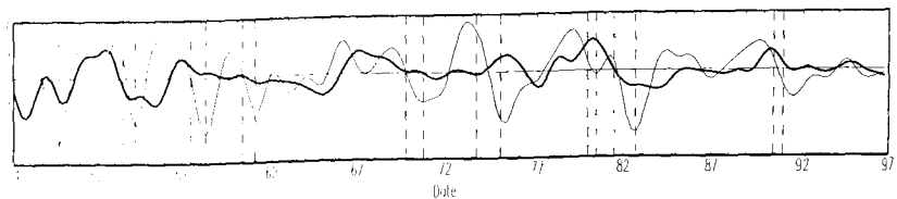
Fig. 3.5. Government employment.
