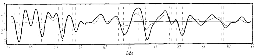
Fig. 3.31. Capacity utilization.
