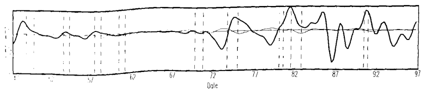
Fig. 3.36. Oil prices.
