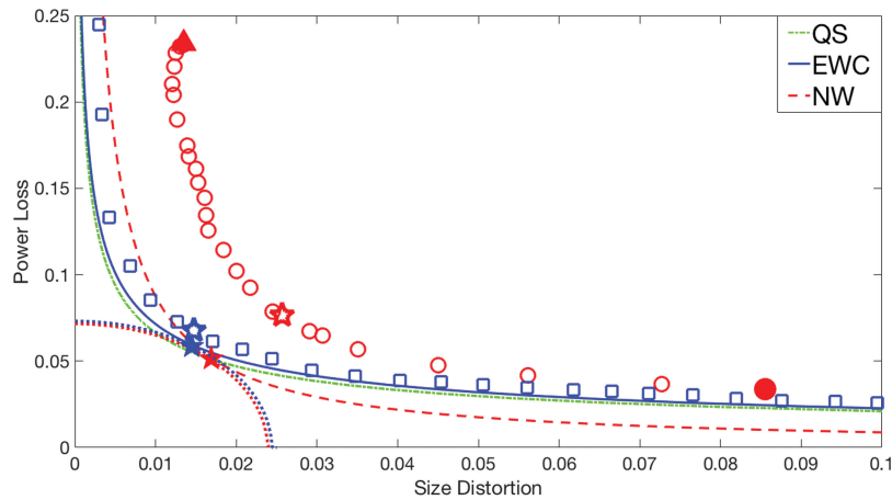
Figure 1. Tradeoff between size distortion, \Delta_S , and maximum size-adjusted power loss relative to the oracle test, \Delta_p^{\max} , T = 200 , in the Gaussian location problem, AR(1) disturbances with autoregression coefficient \rho = 0.7 . Notes: Lines are the asymptotic frontier (green) and the theoretical tradeoffs for the NW test (dash) and EWP/EWC tests (solid); symbols are Monte Carlo values for NW (circle) and EWC (square); solid circle is NW using the Andrews rule S = 0.75T^{1/3} , solid triangle is the Kiefer-Vogelsang-Bunzel (2000) test, ellipses are iso-loss curves ((5) with \kappa = 0.90 ); stars are the loss-minimizing rule outcomes in theory (solid) and Monte Carlo (open).
