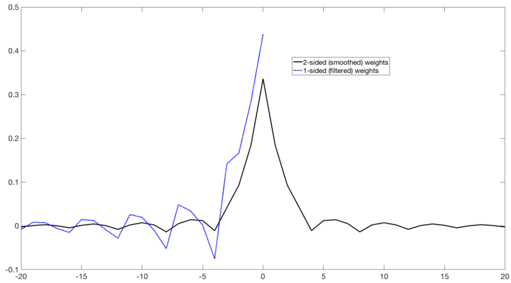
Figure 4: Weight placed on \pi_{+j} for estimating \pi .
