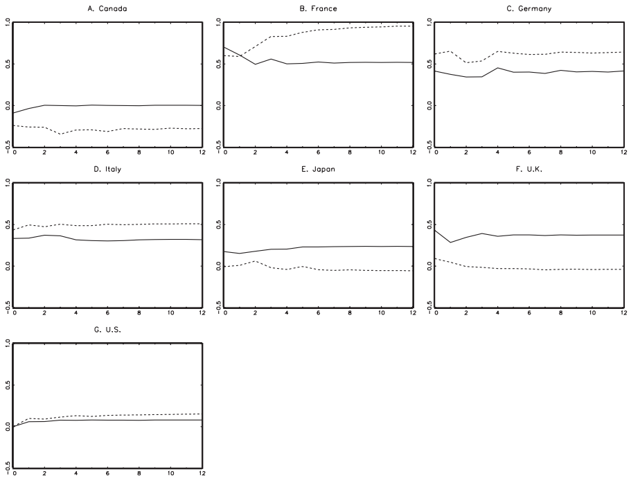
FIGURE 8b. Cumulative impulse response of country GDP growth with respect to the second common factor in 1960–1983 (solid line) and 1984–2002 (dashed line).
