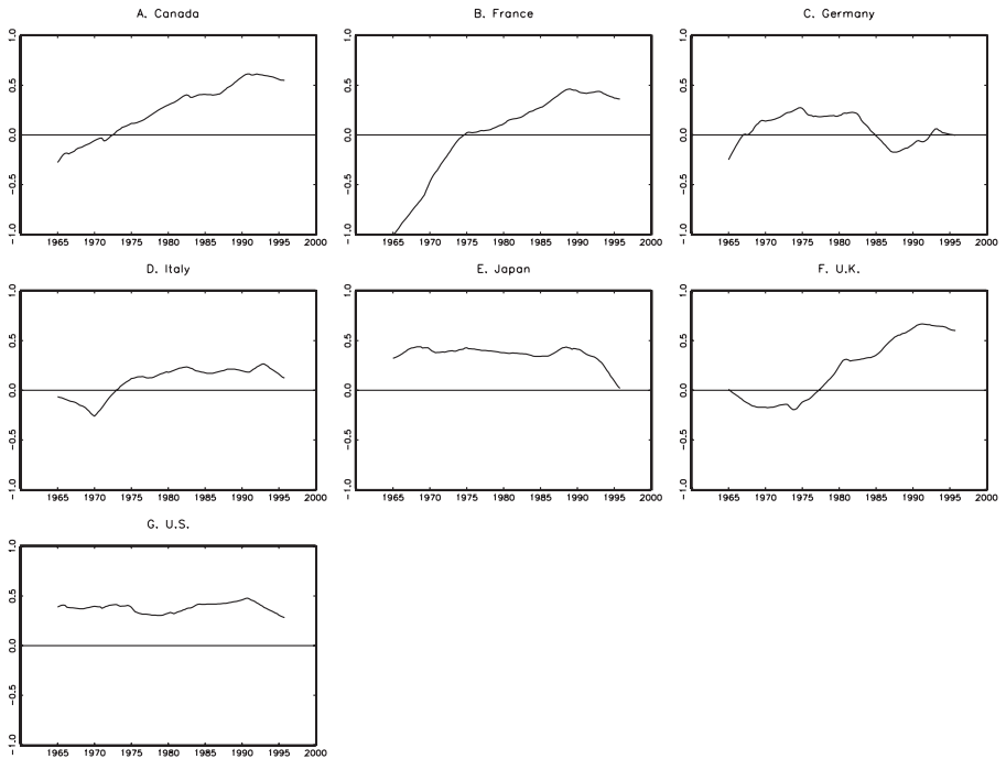
FIGURE 5a. Rolling autoregressions: Sum of AR coefficients ( \hat{\alpha}(1) ).
