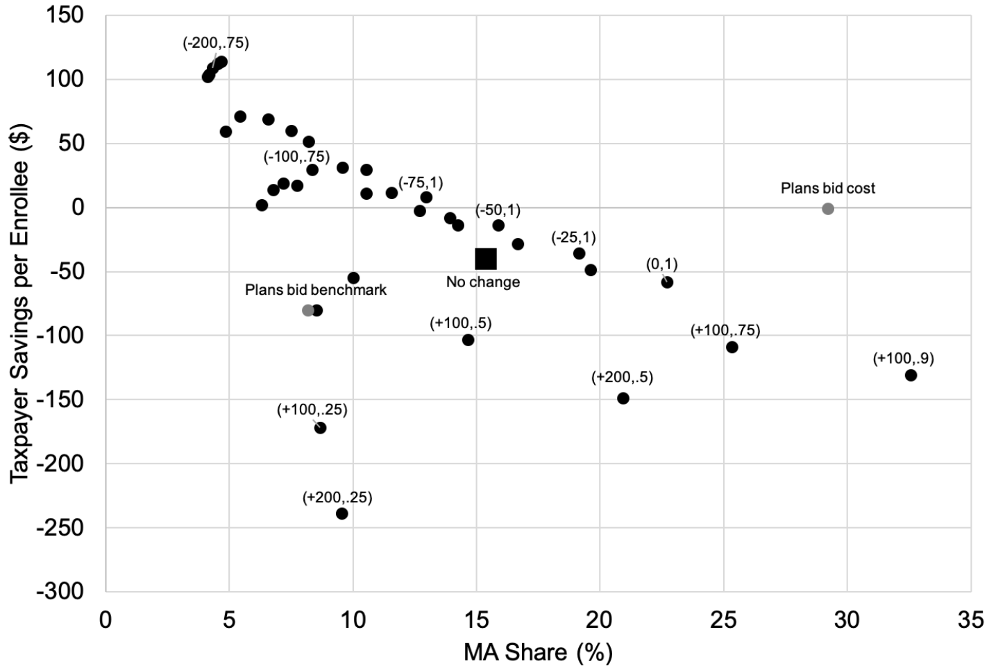
Figure 5: Predicted outcomes under different market design parameters
