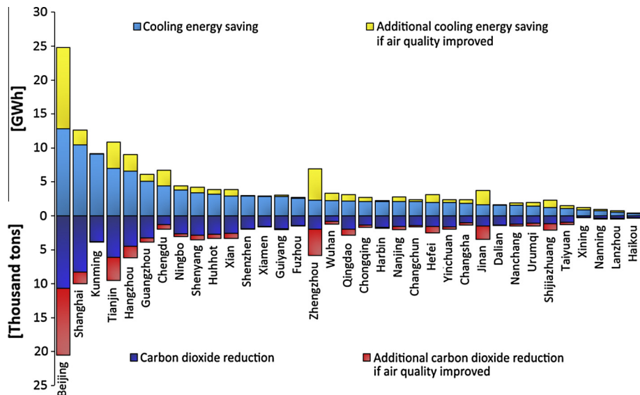
Fig. 5. (Top) energy savings potential and additional cooling energy savings (if air quality is improved) in GWh of 35 major Chinese cities for office buildings ranked from high to low; (Bottom) carbon dioxide reduction potential in thousand tons and the additional cooling energy saving (if air quality is improved) at 35 major Chinese cities for office buildings.
