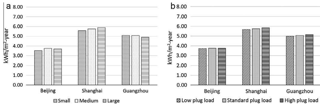
Fig. 6. Per-square-meter cooling energy savings by natural ventilation: (a) small, medium, and large building; (b) low internal load (10 W/m 2 ), baseline plug load (15 W/m 2 ), and high internal load (20 W/m 2 ) in Beijing, Shanghai and Guangzhou.
